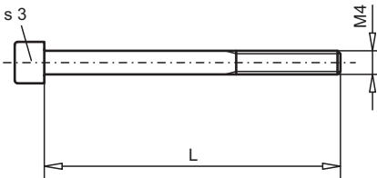
SOCKET HEAD CAP SCREW M4xL
