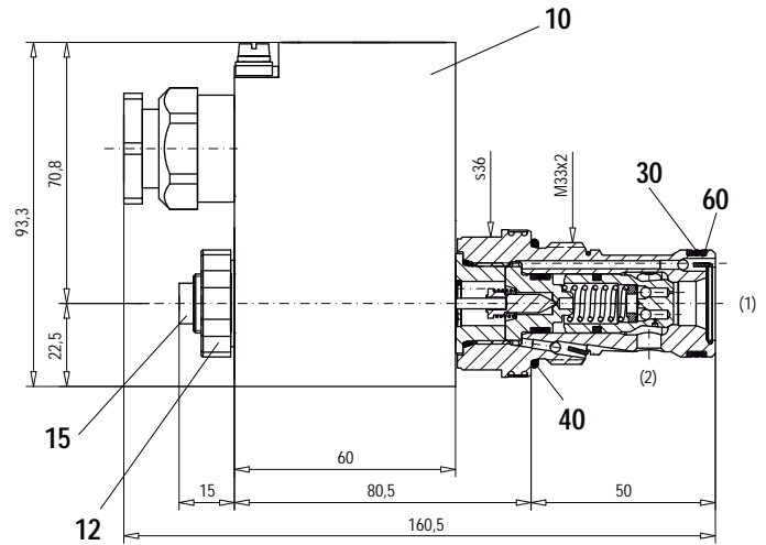
2/2-way version, «normally closed» [BA]
